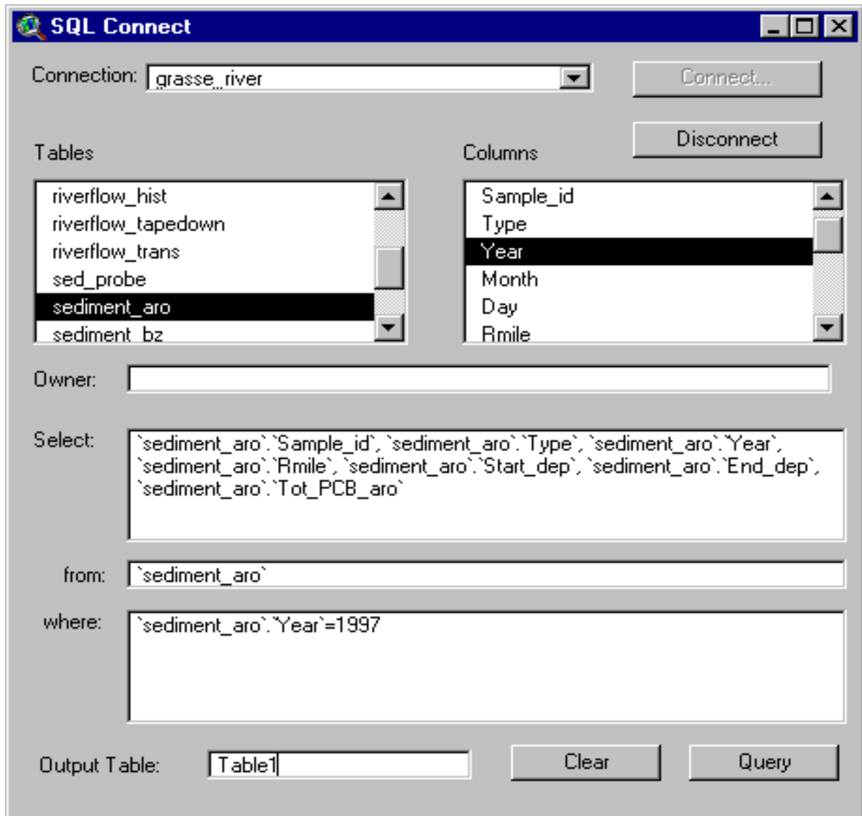
Figure 2-1. SQL connect window.
